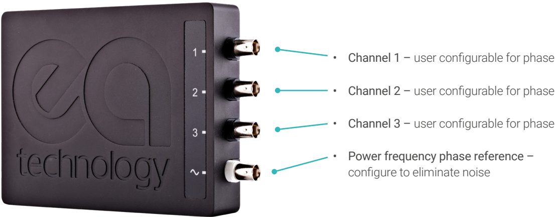
Figure 7: CableData® Collector central unit
