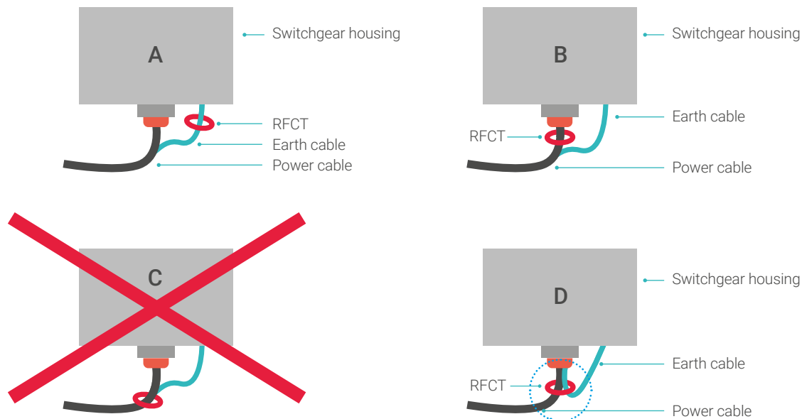
Figure 10: Cable Connection Methods
