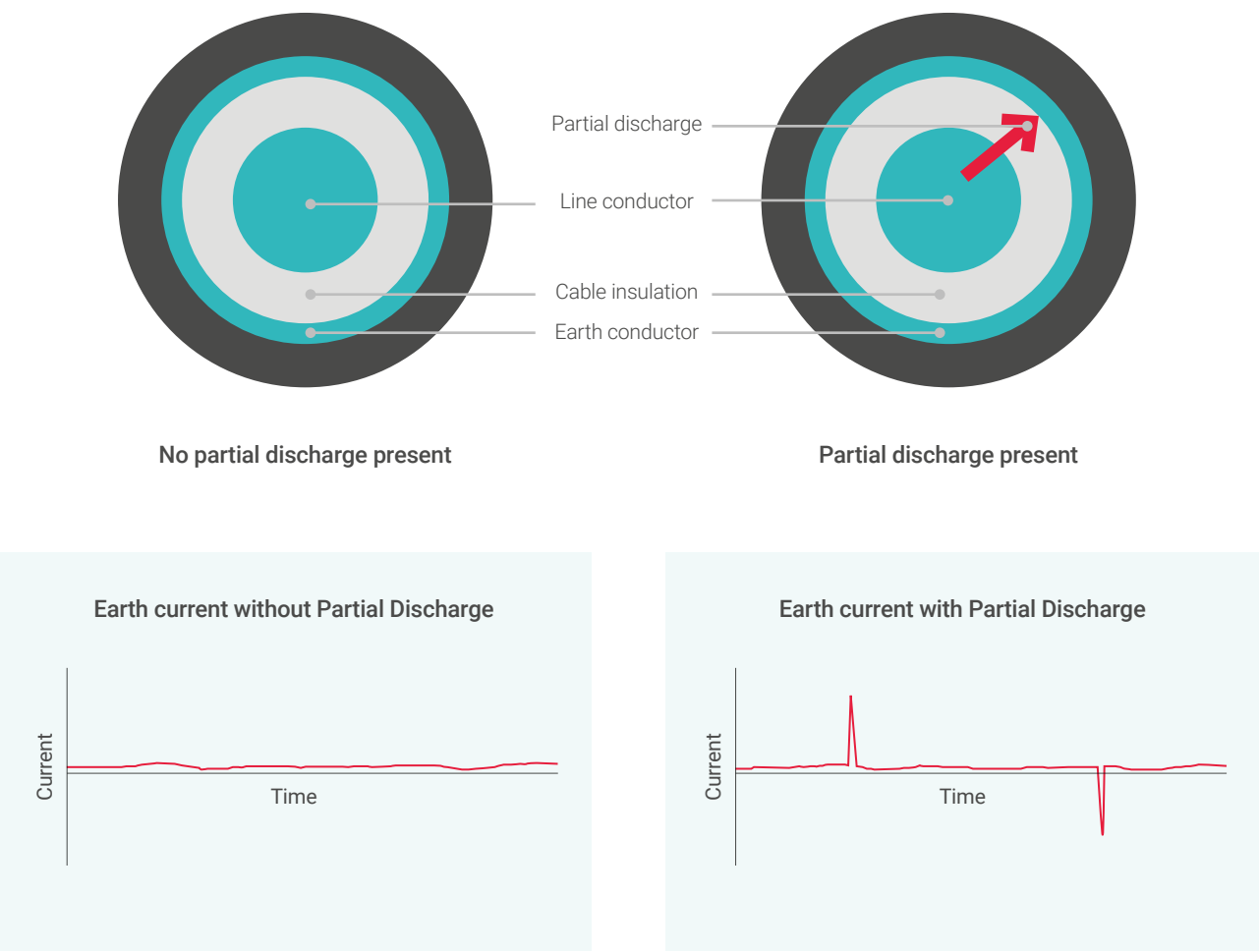
Figure 9: Effect of Partial Discharge on a cable
