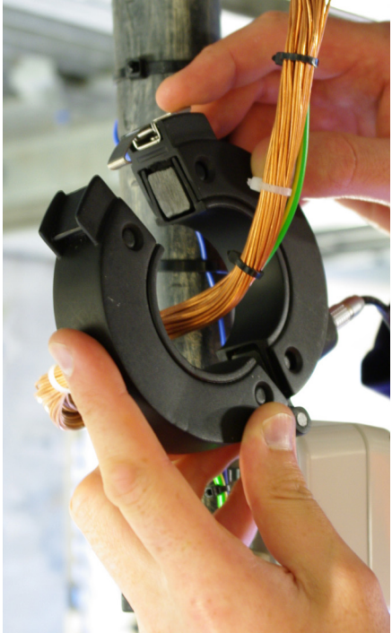
Figure 6: RFCT on earth braid of HV cable
